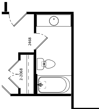
BEDROOM 4 BATH
