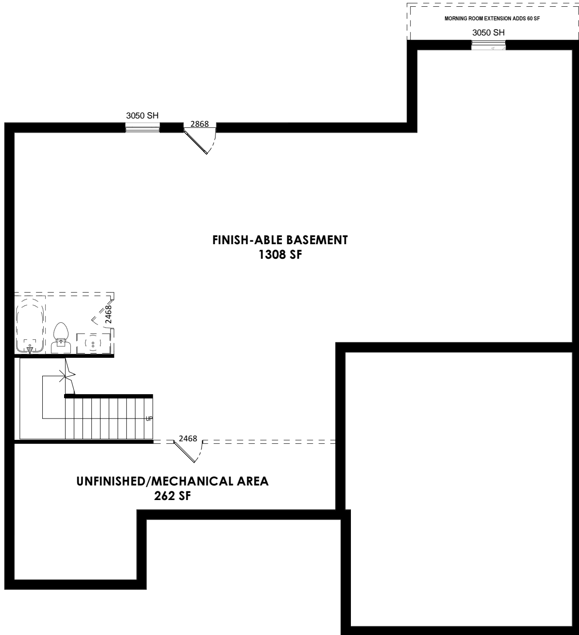
BASEMENT PLAN
